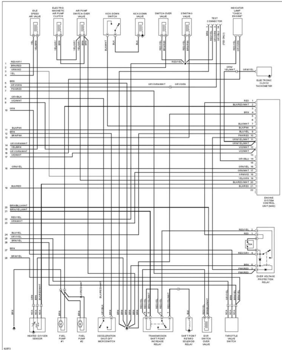
Fig. 8: 3.0L, Engine Performance Circuits (2 of 2)
